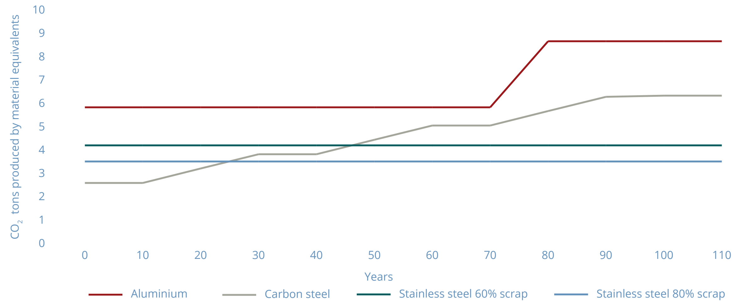
Figure 5 CO 2 production emissions for alloys in structures over 110 years of operational life The data was calculated from material and processing emissions data available from the world stainless association, the World Steel Association and the Organisation for Economic Co-operation and Development (OECD).
