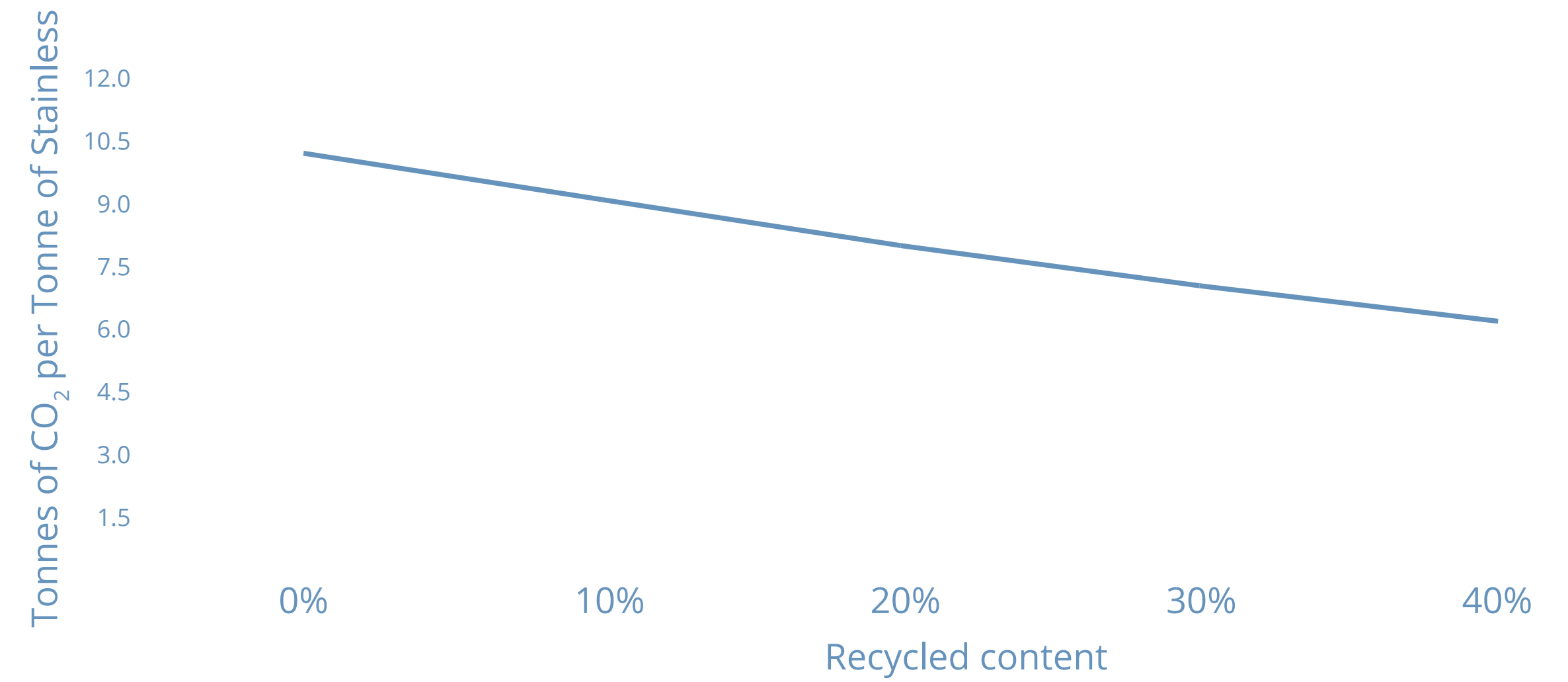
Figure 4 Calculated CO 2 Emissions for NPI-Based Production Data source: worldstainless, 2023
