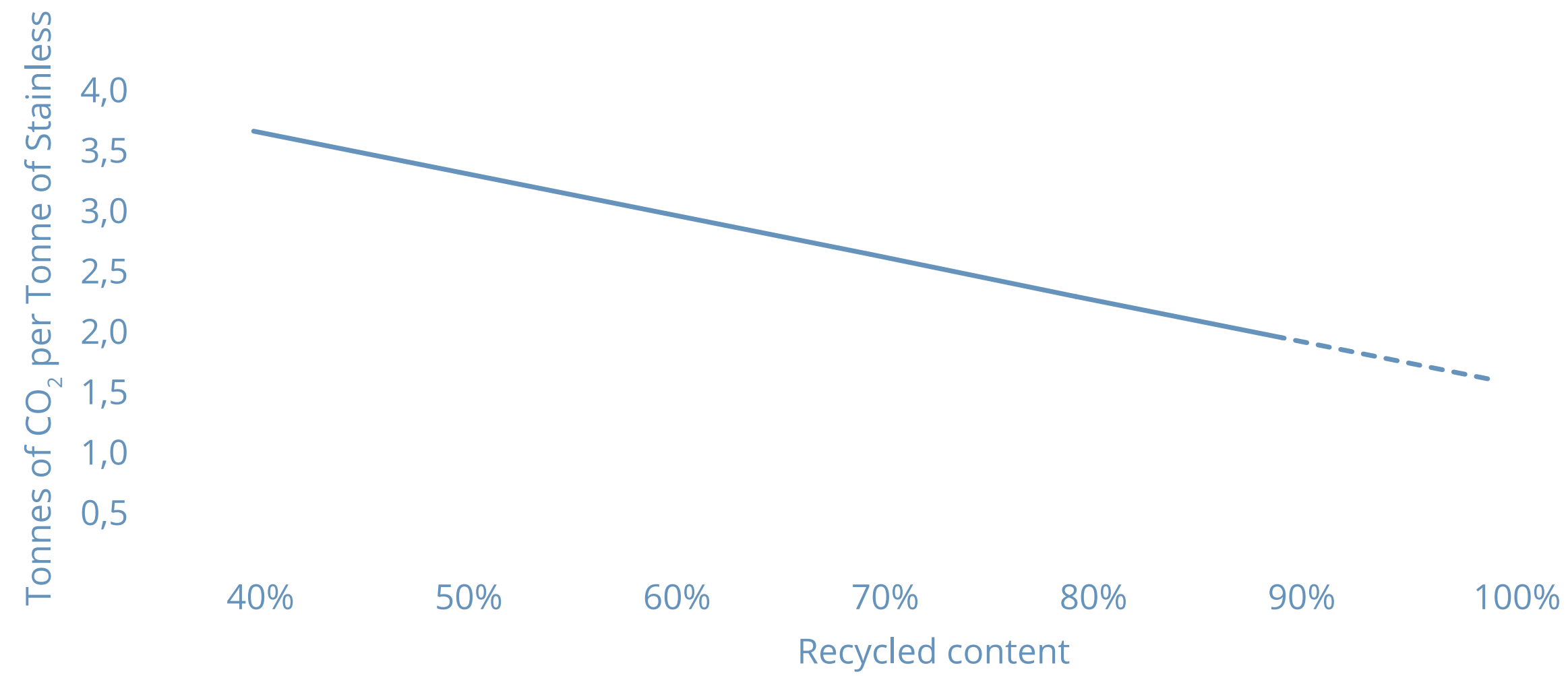
Figure 3 Actual CO 2 Emissions for Scrap-Based Production Data source: worldstainless, 2023
